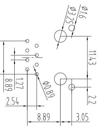
PC Board Layout Component Side Shown
